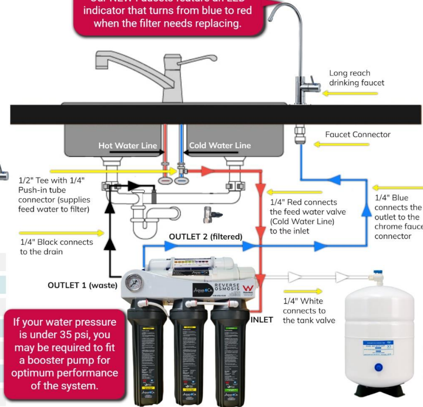
USA Reverse Osmosis System
