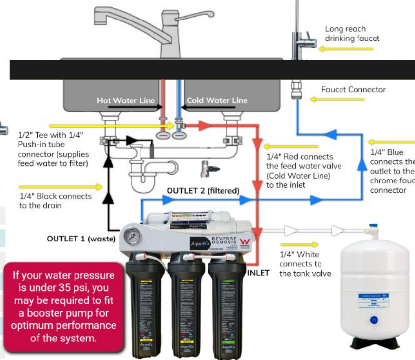
USA Reverse Osmosis System
