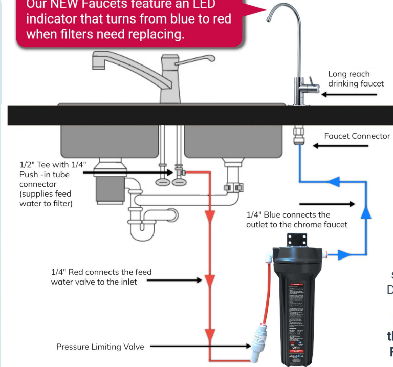
Single Undersink System w/ Aragon Filter
